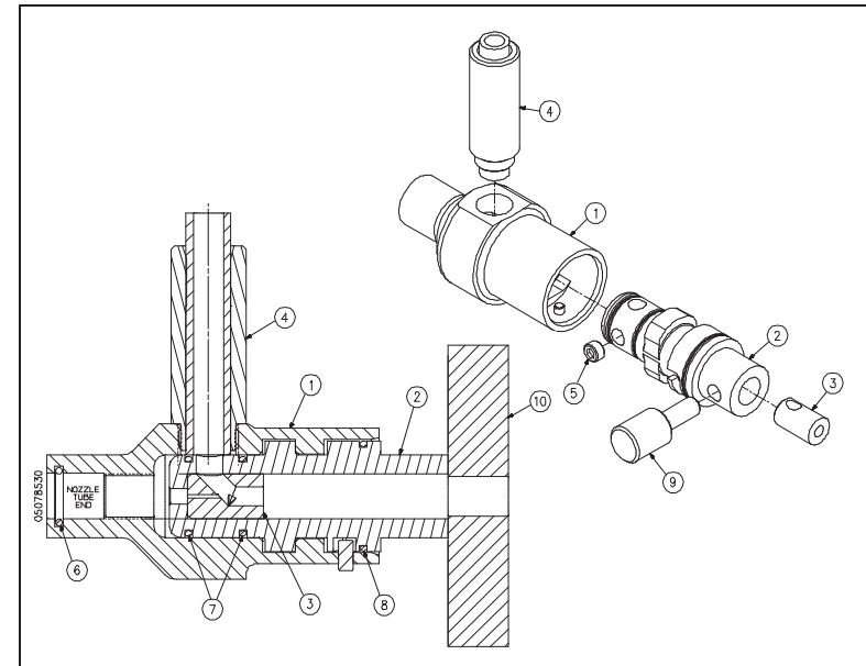
Figure 12-34: Autoline™ Abrasive Nozzle Assembly
